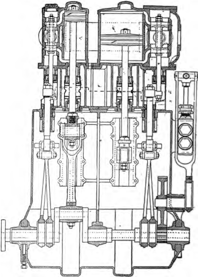
FIG. 379.—The "Lifu" Compound Steam Engine for heavy vehicle use. This section is drawn through the centre of the cylindrical steam chests, which, as in the Thornycroft engine (Fig. 377), are below and at the sides of the steam cylinders. The appearance of eccentricity in the attachment of the piston-rods may thus be understood.
